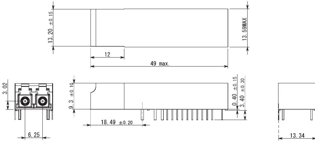
Figure 2-1. Outline Dimensions(SCM6002-GL-ZN)
