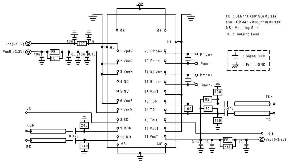
Figure 5. Recommended Interface Circuit
