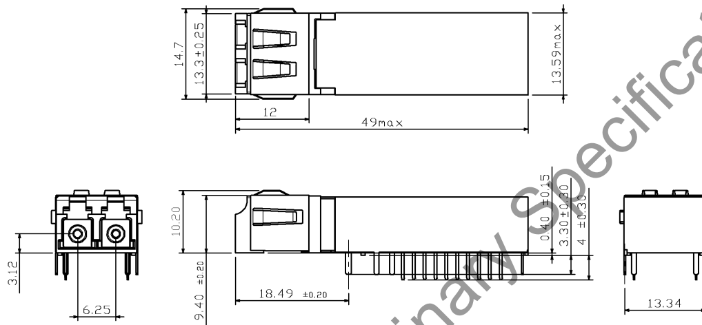
Figure 2-2. Outline Dimensions (SCM6008-GL-CN)
