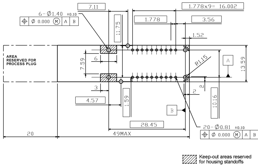
Figure 2-3. Recommended Footprint
