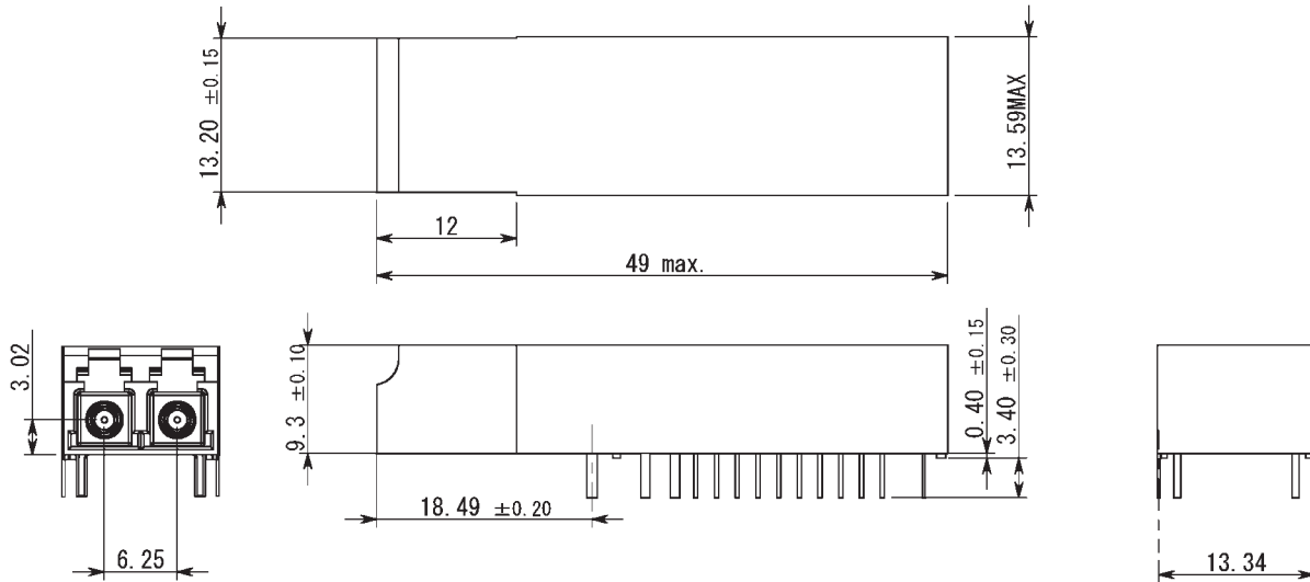
Figure 2-1. Outline Dimensions(SCM6011-GL-ZN)
